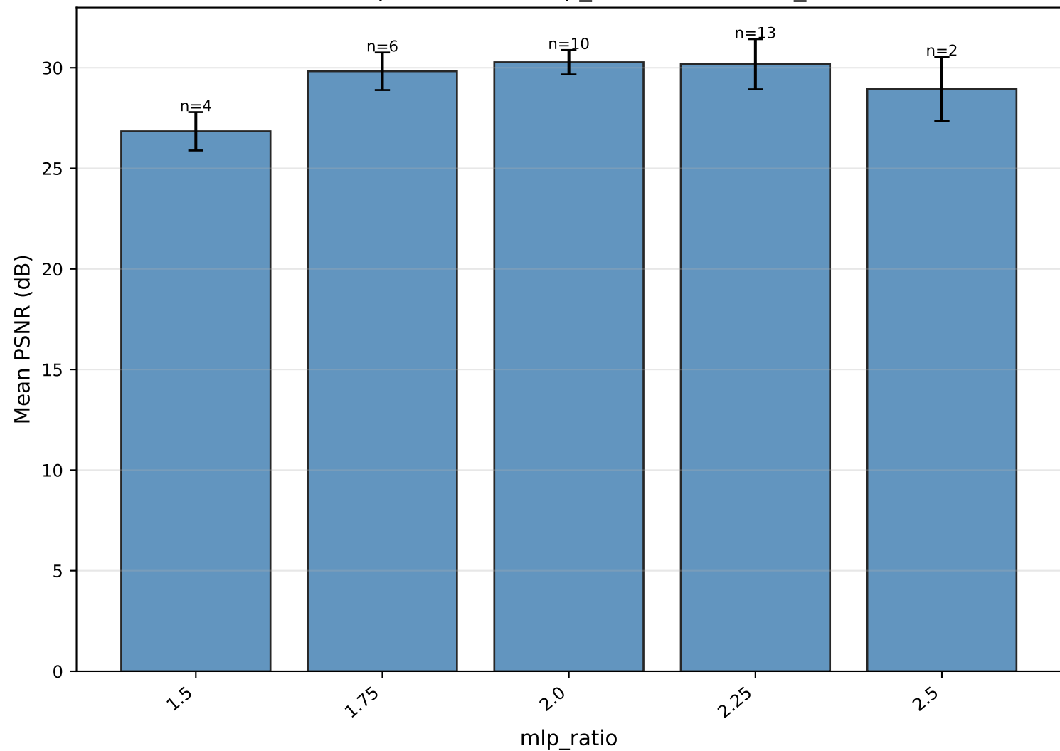
Mean PSNR per value of mlp_ratio — DHTCUN_baseline
